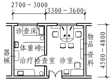
套间诊疗室(24m 2 )
